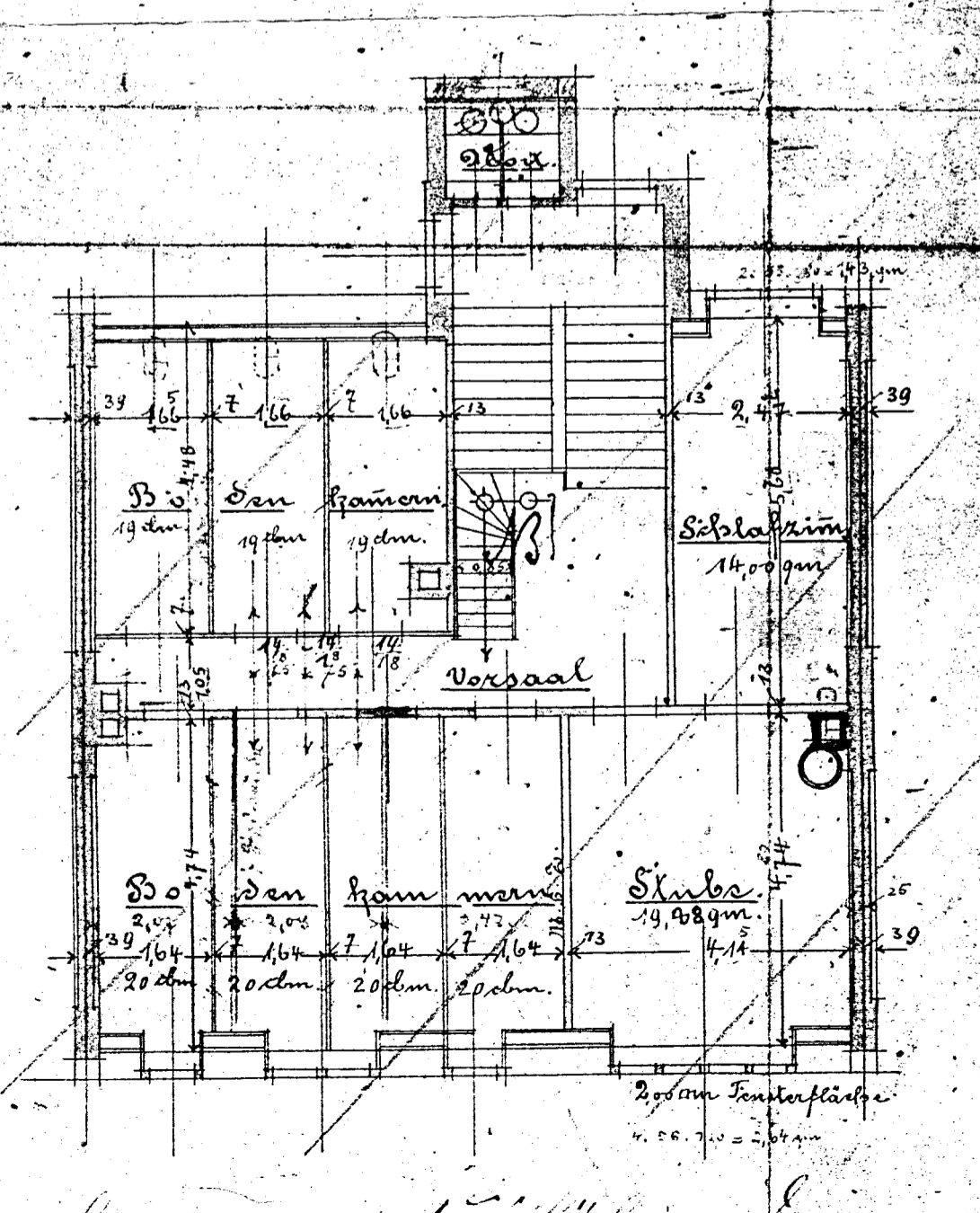
Dach = Erdgeschoss.
